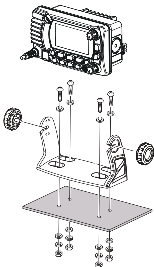
Desktop Mounting
