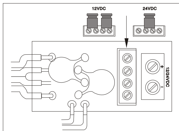
Wiring Instructions
