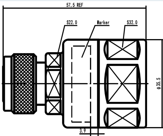
43MH-LCF78-C03 Outline drawing
