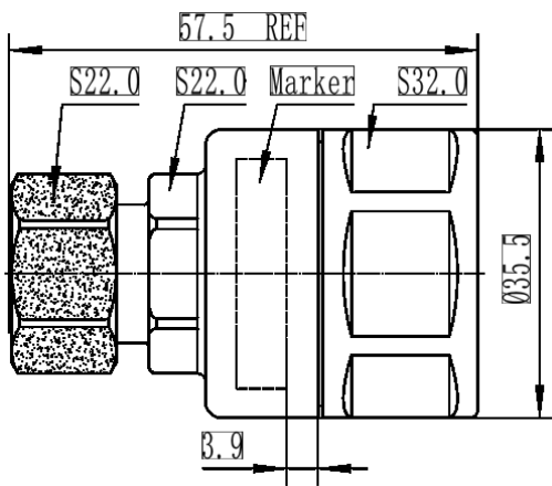
43M-LCF78-C03 Outline Drawing
